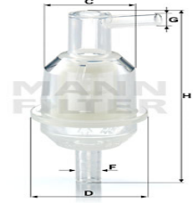
Fuel Filter WK 31/5 EM-20028
